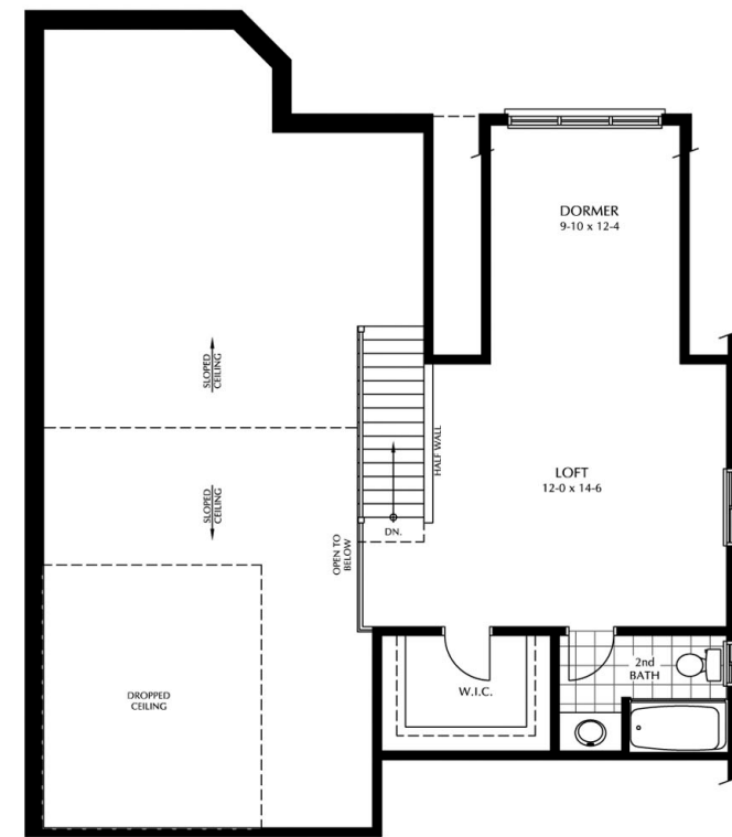
OPTIONAL LOFT LOFT FLOOR AREA - 545 sq.ft.
