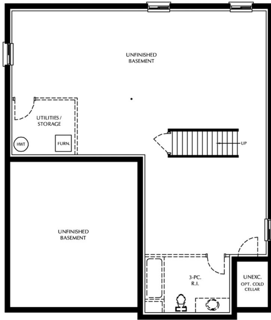
BASEMENT PLAN
